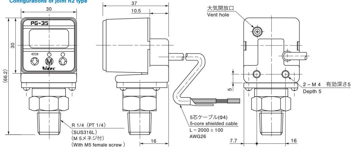
継手形状 R2タイプ Configurations of joint R2 type
